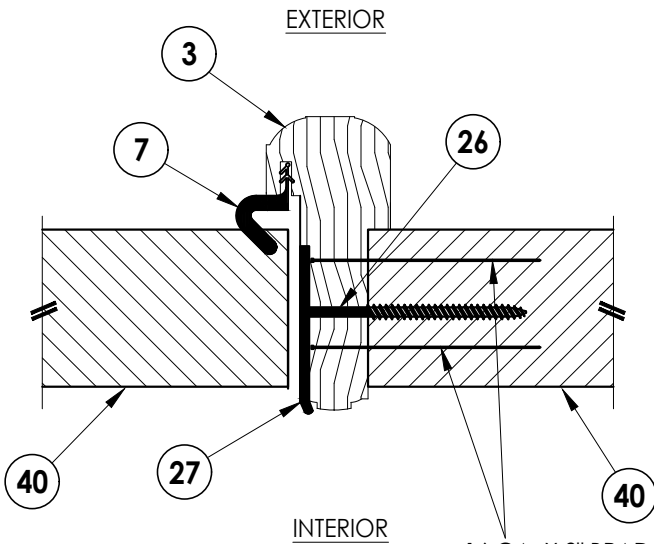
3 HORIZONTAL CROSS SECTION Inswing shown (Outswing similar)
